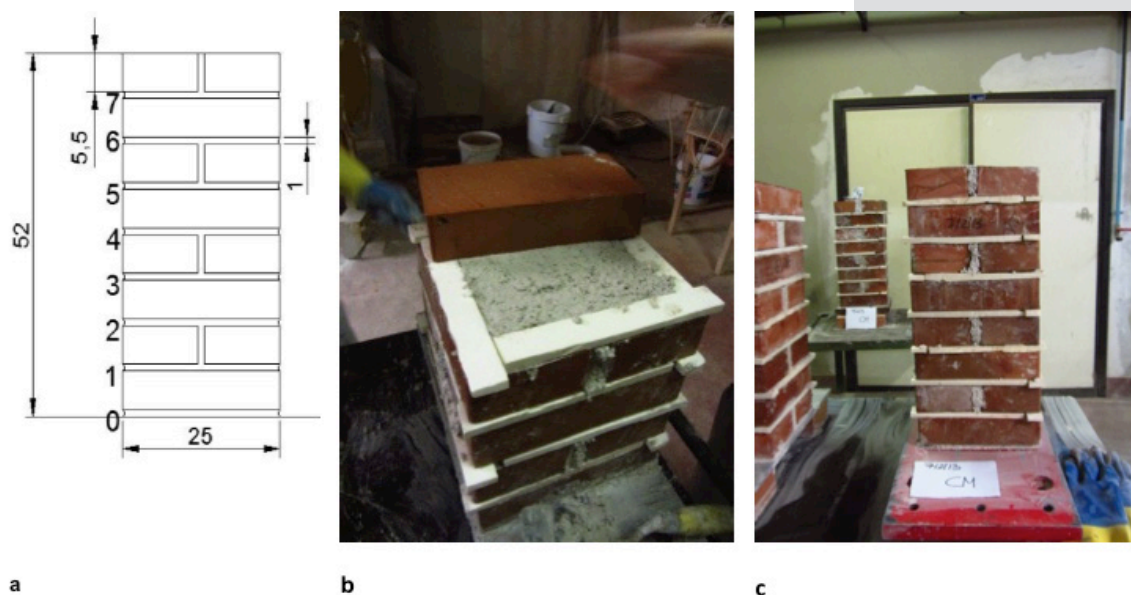
Figure 2. Metric survey (values in cm) of the specimen (a) – The use polystyrene during the samples manufacturing (b and c).
