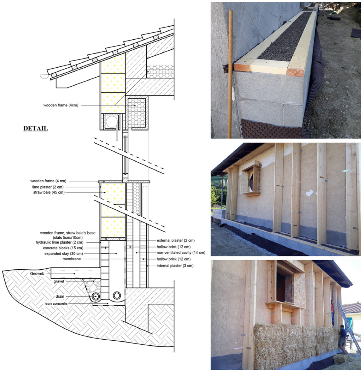
Fig. 5. Wall section detail and a photo of the construction site.
