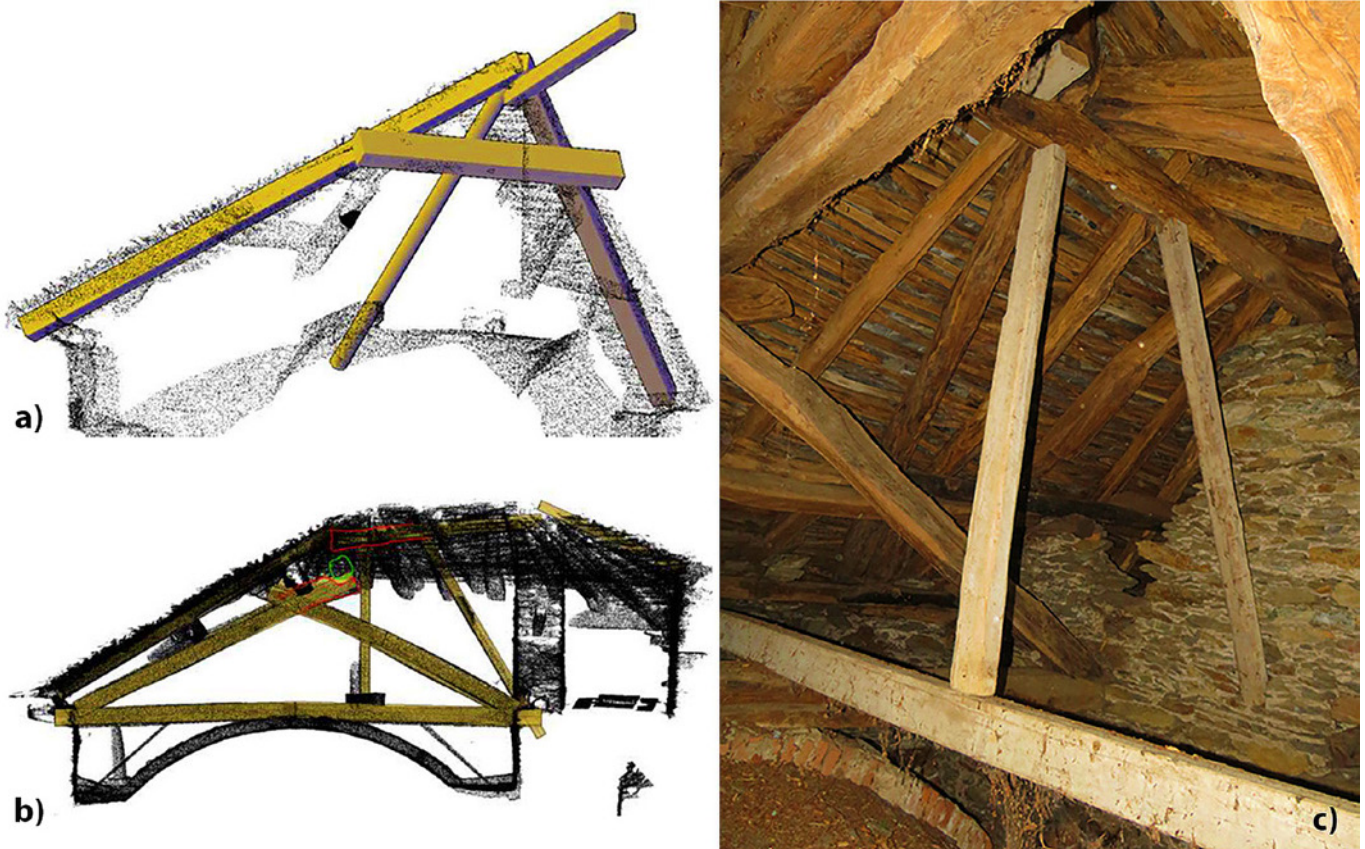
Fig. 6. (a) Laser scanner survey of the roof area, including the two cantonal beams; (b) hypothesis of the original configuration of the ridge beam; (c) props to support the ridge beam.
