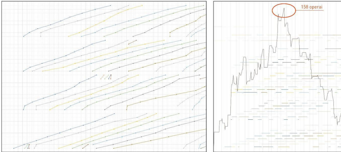
Figure 10) An overview of the line of balance of the site and the issue highlighted in the productivity graph. 1
