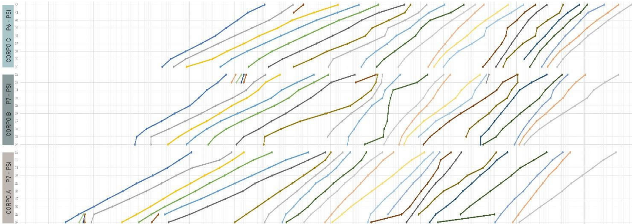
Fig. 09) an extended view of CPG line of balance, derived from the ABM process. 1
