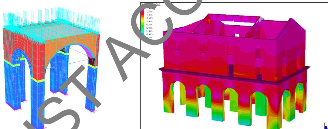
Figure 5 – Exemplary representation of the F.E.M. model of the "local significant module" (axonometric view of structural elements, loads and nodes) and "global model" (axonometric view of the structural analysis results - ZZ stresses).
