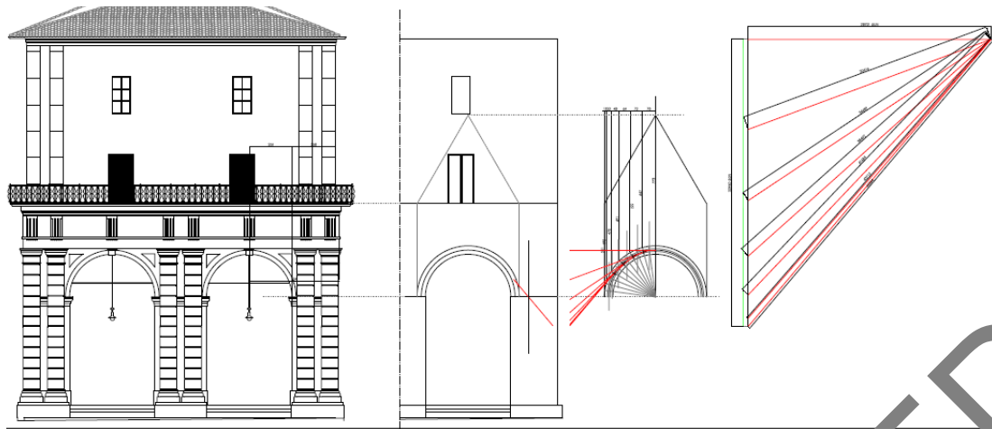
Figure 4 – Search for the "A2" arch pressure line.
